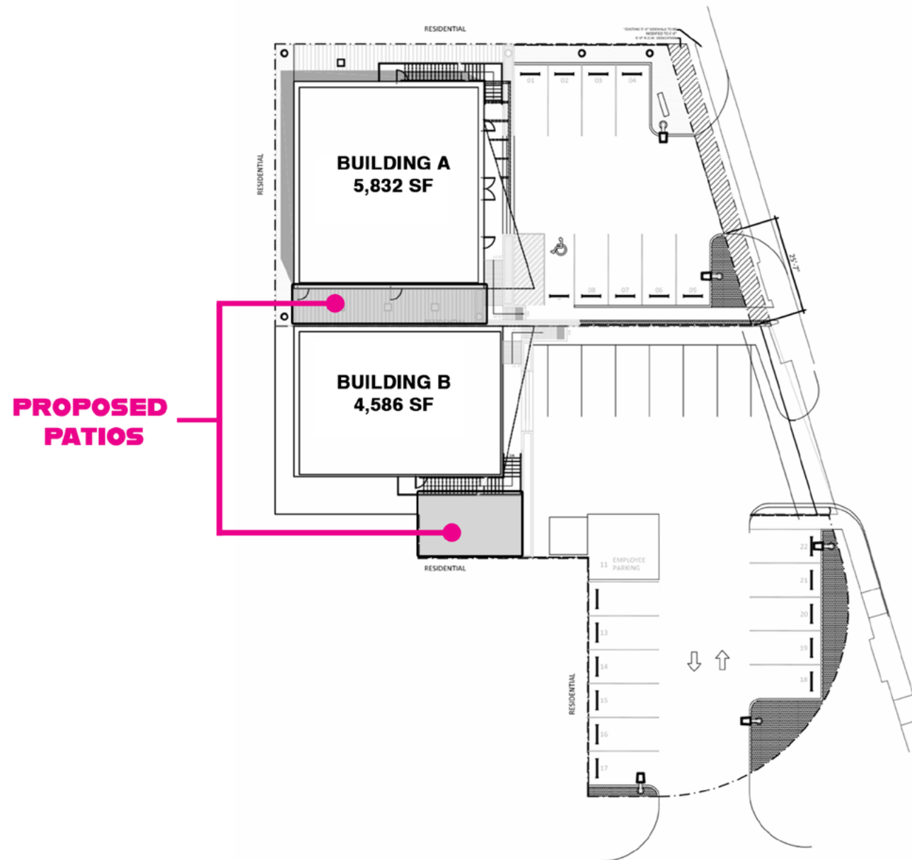
MODERNE @ MAIN SITE PLAN
